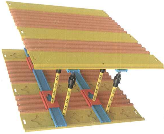
2.52m deep x 3.0m wide EZE Shoring System
